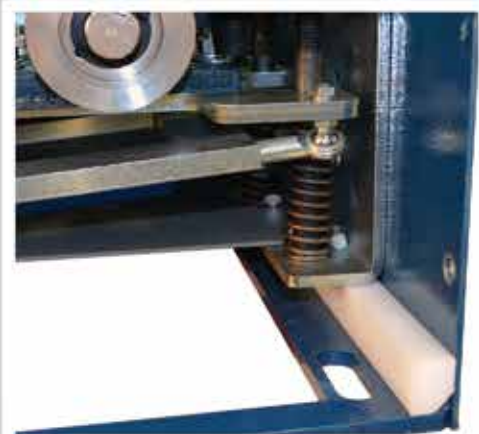
Spring mounted suspension that moves with rail
