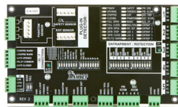
LOGIC BOARD
