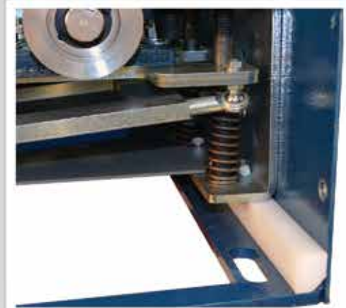
Spring mounted suspension that moves with rail
